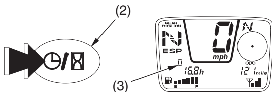
(2) digital clock/hourmeter select button
